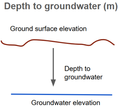
Figure 10. A simplified graphic depicting how depth to groundwater (DTG) is calculated using ground surface and groundwater elevations.
