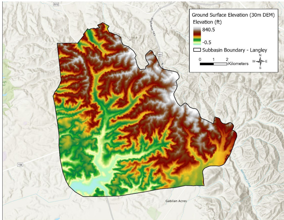
Figure 3. Digital Elevation Model (DEM) ground surface elevation (feet) in the Langley Area Subbasin (USGS 2024).
