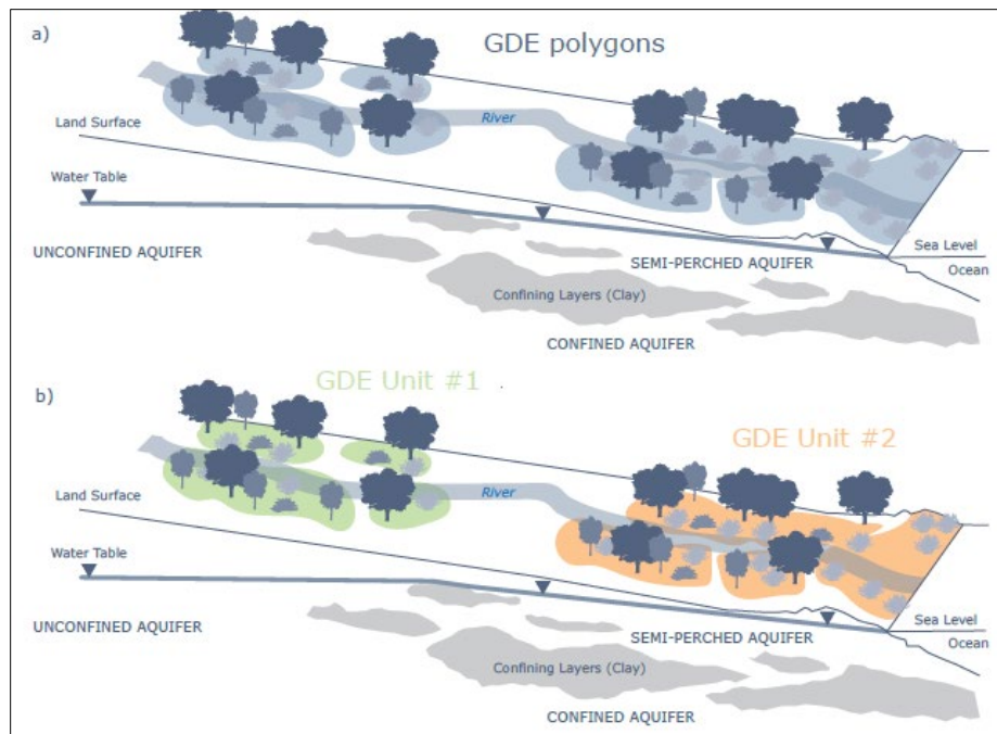
Figure 8. Illustration of grouping GDEs into units based on shared association with an aquifer. a) GDEs not separated into units, b) GDEs separated into two units, Unit #1 is associated with an unconfined aquifer, Unit #2 is associated with a “semi-perched aquifer” above a confined aquifer. Image Credit: Rhode et al. 2018
