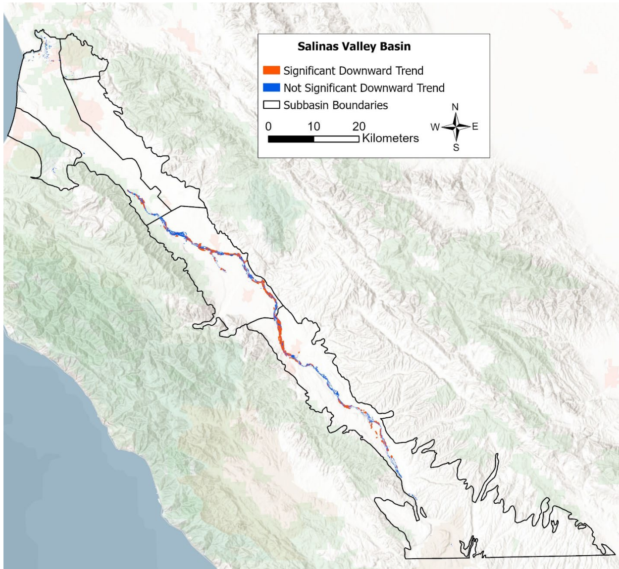
Figure 14. Salinas Valley GDE trends. Potential GDEs with a statistically significant negative relationship between Z_{NDVI} and Z_{DTG} (significant downward trend) are in orange, potential GDEs that did not have a significant downward trend are in blue. The symbology for significant downward trends (orange) is enlarged for visibility.
