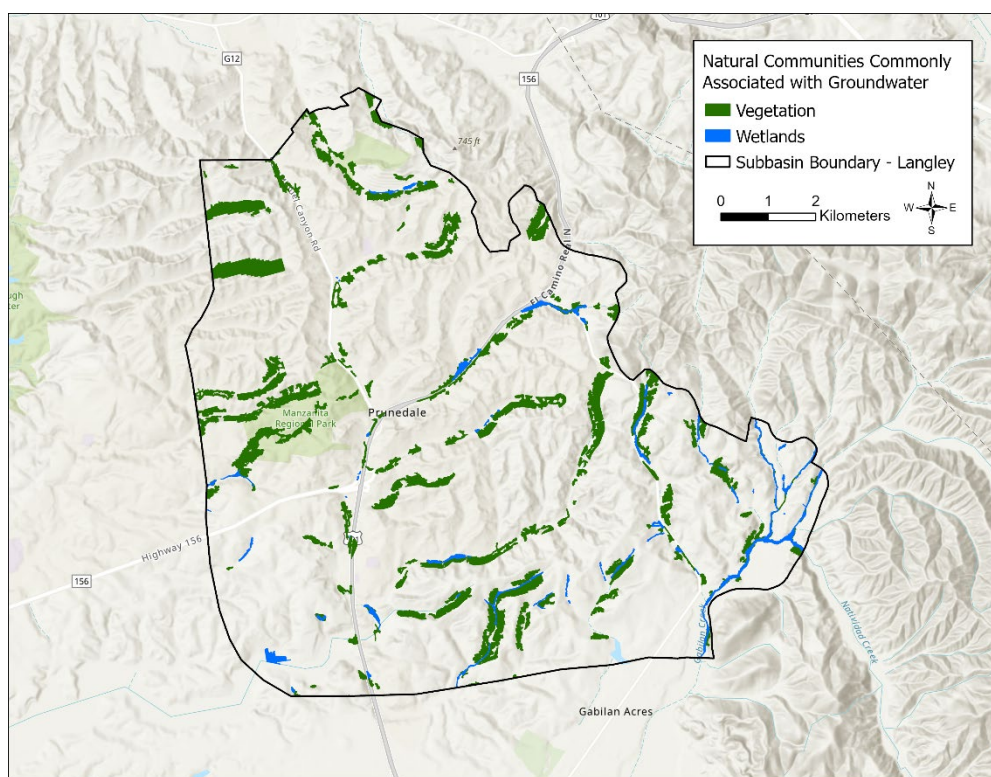
Figure 1. Natural Communities Commonly Associated with Groundwater dataset focused on the Langley Area Subbasin (Klausmeyer et al. 2018).
