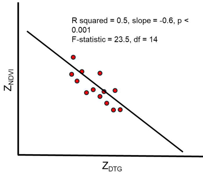
Figure 11. Illustrative example, not based on real data, of the linear model generated for each GDE based on NDVI and DTG Z-scores calculated for each available year (15 years for which data from both datasets were available). This example describes a statistically significant negative relationship between NDVI and DTG, due to the negative slope of the best fit line and a p-value of < 0.001 .
