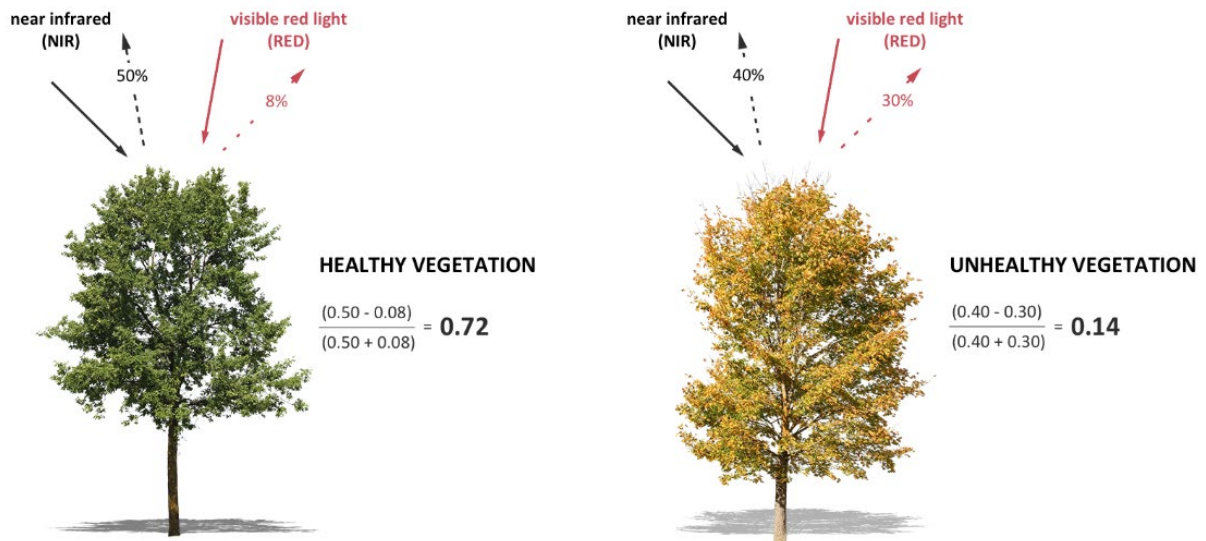
Figure 9. This graphic depicts how NDVI is calculated and gives an example of how much light is absorbed versus reflected by healthy, green vegetation compared to unhealthy, less green vegetation. As vegetation greenness declines, the percentage of reflected light increases (image credit: TNC 2024).
