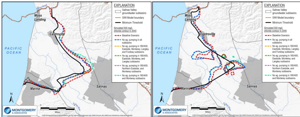
Figure 4. 180 and 400-Foot Aquifers Modeled SWI at 2040
