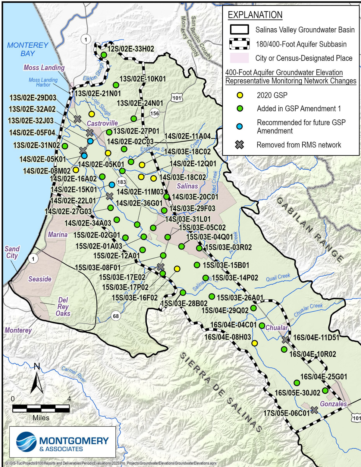
Figure 5-2. 400-Footer Aquifer Groundwater Elevation Representative Monitoring Network Changes
