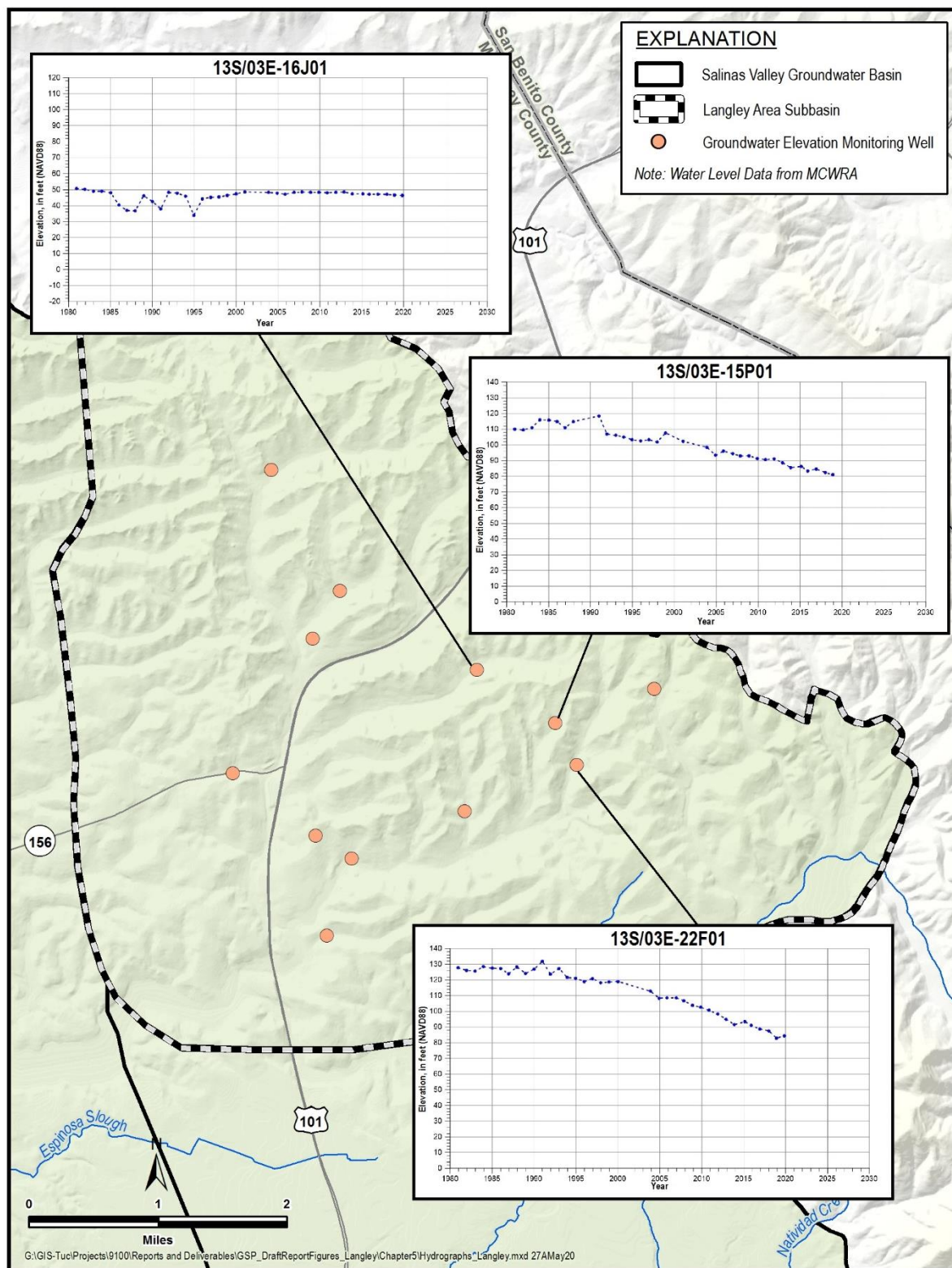
Figure 1. Monitoring Wells and Example Hydrographs
