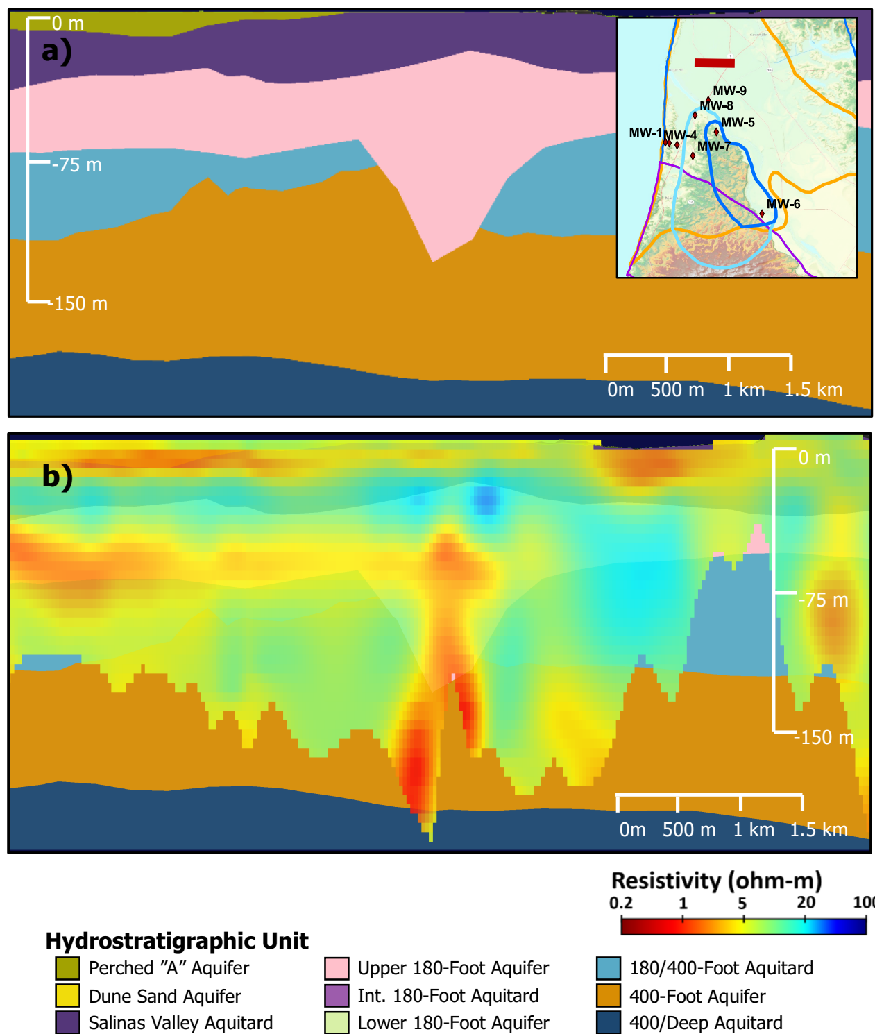
Figure 14: Determining gaps in the 180/400-Foot Aquitard from AEM data. Above, a) shows a cross-section of the post-AEM model based on cross-sections from previously published reports, with an inset map showing the approximate cross-section location as a red bar. Below, b) shows the same post-AEM model with the AEM resistivity model superimposed. Opacity of the AEM resistivity model is set to approximately 80%.
