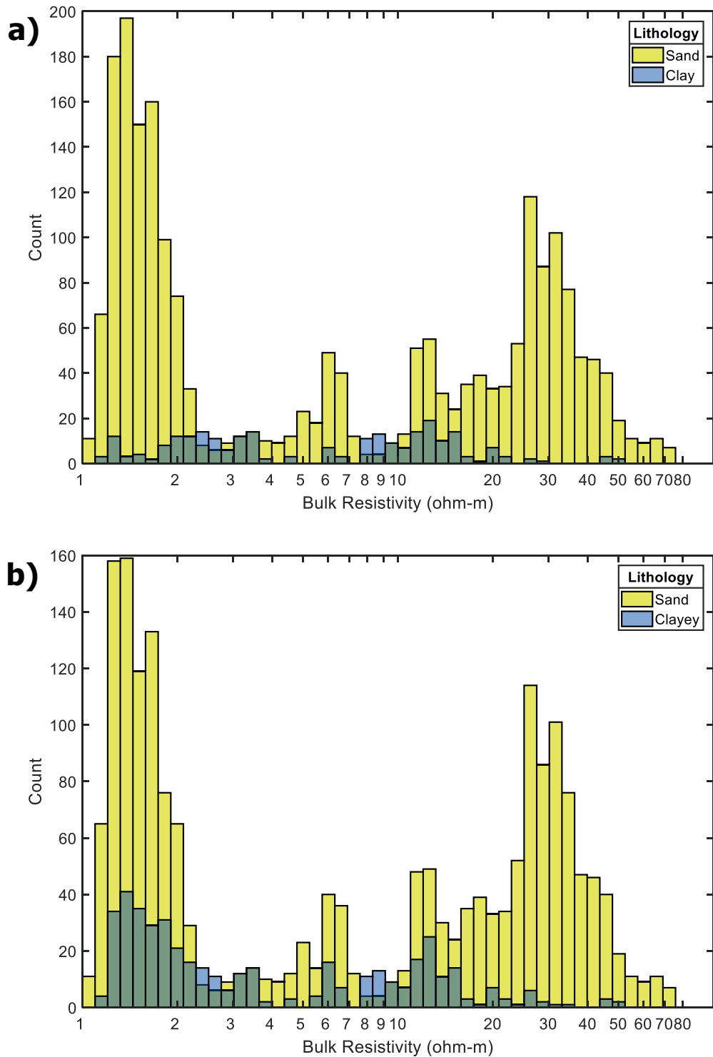
Figure 13: Resistivity values from geophysical measurements in MPWSP monitoring wells, colored according to a binary lithology classification. In a) all values are colored yellow, aside from any lithology descriptor containing the word "clay", which are colored blue. In b) the values colored blue are expanded to include any lithology descriptor including the word "clay" or "clayey". Regions where blue bars overlap yellow bars appear blue-green.
