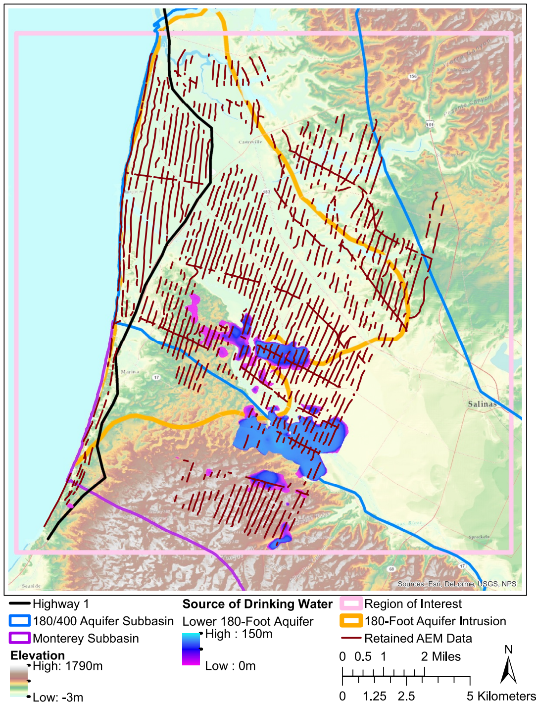
Figure 24: Interpreted thickness of the subsurface containing sources of drinking water within the Lower 180-Foot Aquifer in the region of interest, shown in a color scale ranging from purple to light blue, representing 0 m to 150 integrated meters of the source of drinking water, respectively. Overlaying the thickness of sources of drinking water are the locations where AEM data were collected and retained for processing, shown as red lines. The extent of saltwater intrusion in the 180-Foot Aquifer, as measured by the Monterey County Water Resources Agency, is shown as an orange line. The boundaries used in calculating the regions containing sources of drinking water, Highway 1, the 180/400 Aquifer Subbasin, and the Monterey Subbasin, are shown as black, blue, and purple lines, respectively.
