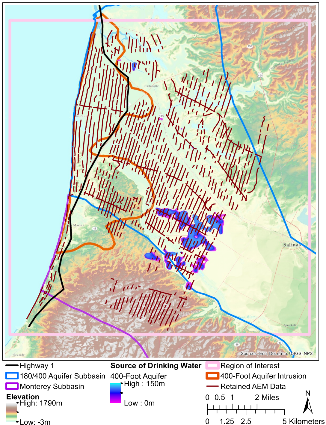
Figure 25: Interpreted thickness of the subsurface containing sources of drinking water within the 400-Foot Aquifer in the region of interest, shown in a color scale ranging from purple to light blue, representing 0 m to 150 integrated meters of the source of drinking water, respectively. Overlaying the thickness of sources of drinking water are the locations where AEM data were collected and retained for processing, shown as red lines. The extent of saltwater intrusion in the 400-Foot Aquifer, as measured by the Monterey County Water Resources Agency, is shown as an orange line. The boundaries used in calculating the regions containing sources of drinking water, Highway 1, the 180/400 Aquifer Subbasin, and the Monterey Subbasin, are shown as black, blue, and purple lines, respectively.
